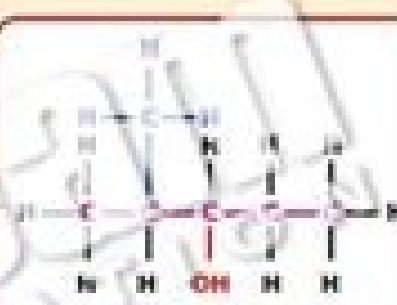
2-Methylpentan-3-ol
